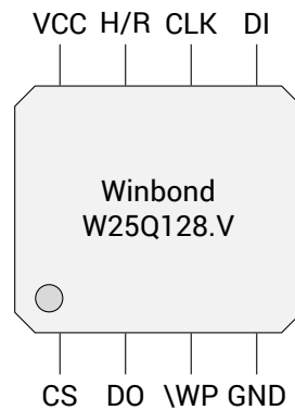
Figure 1: the pin-out of the Winbond W25Q128.V SPI NOR flash
