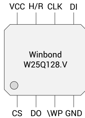
Figure 2: the pin-out of the Winbond W25Q128.V SPI NOR flash
